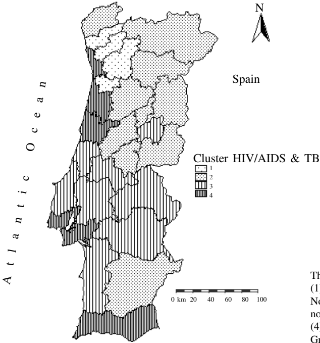
Figure 3 Hierarchical ascending classification. Clusters, males
